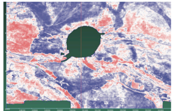
Stratal domain.
