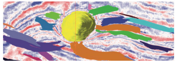
Structural domain.
