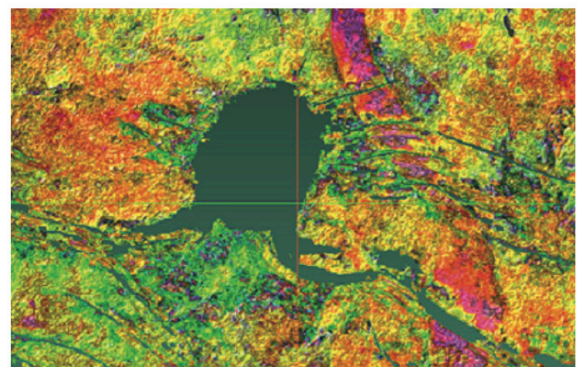
Stratal domain.
